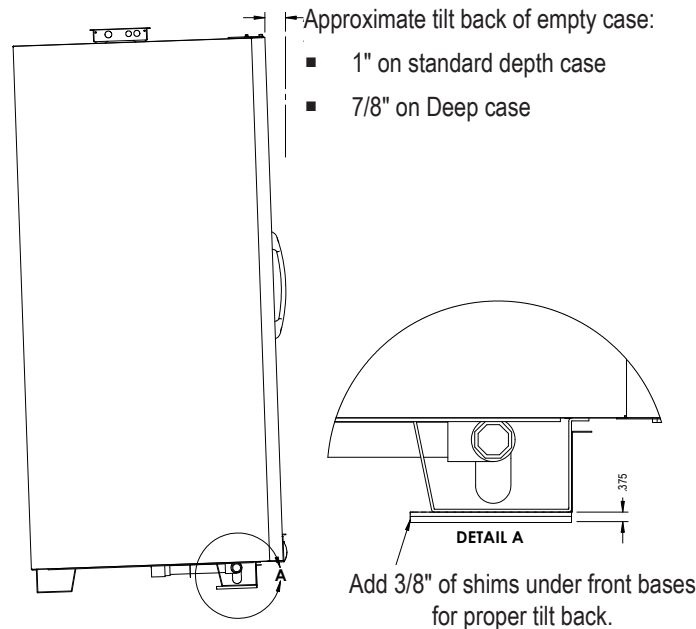
FIGURE 14: Tilt Back
