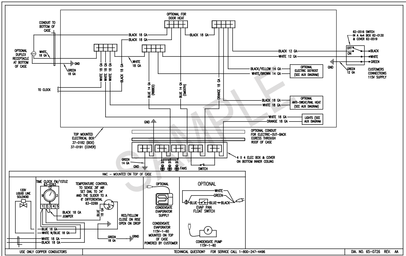
FIGURE 39: Sample Wiring Diagram
